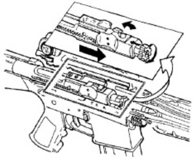
Figure 2-13. Locking.
